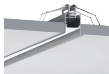
Installed Spring Clip
